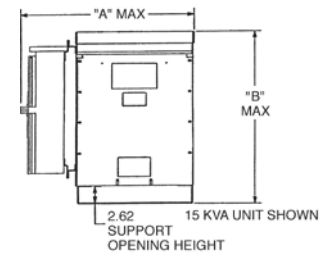
Dimensions Three-Phase
