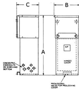
Dimensions Single-Phase
