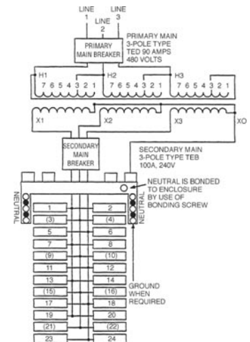
Typical Wiring Diagram Three-Phase 1
